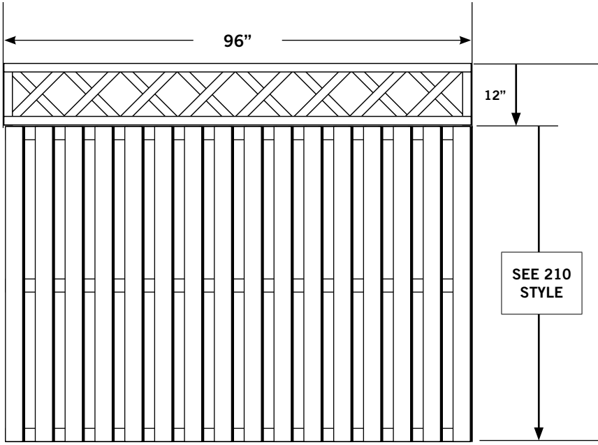
800-1 Lattice Topper
