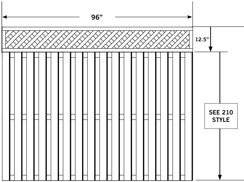
215-1 Lattice Topper
