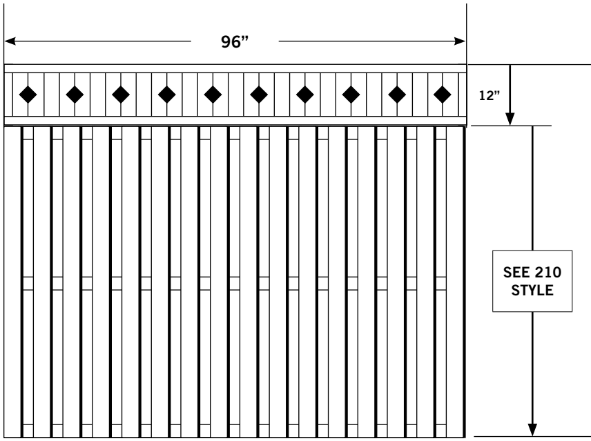
400-1 Lattice Topper
